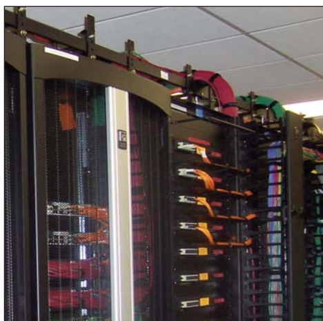
Multiple F-Series TeraFrame™ Cabinet Systems equipped with CPI Passive Cooling™ Solutions populate OMI's center data center.
