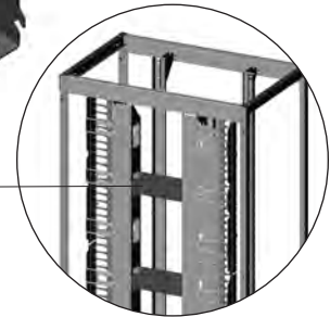
Front-To-Back Cable Manager installed
