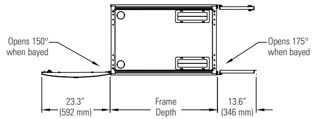
Top View (Server Top Panel without Vertical Exhaust Duct Knockout)
