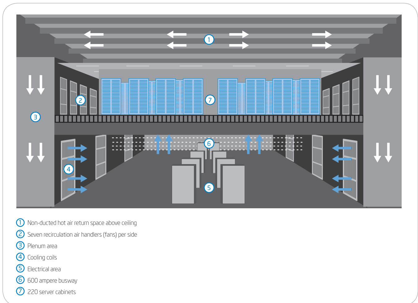
Figure 3. Cross section of a two-story high-performance data center.
