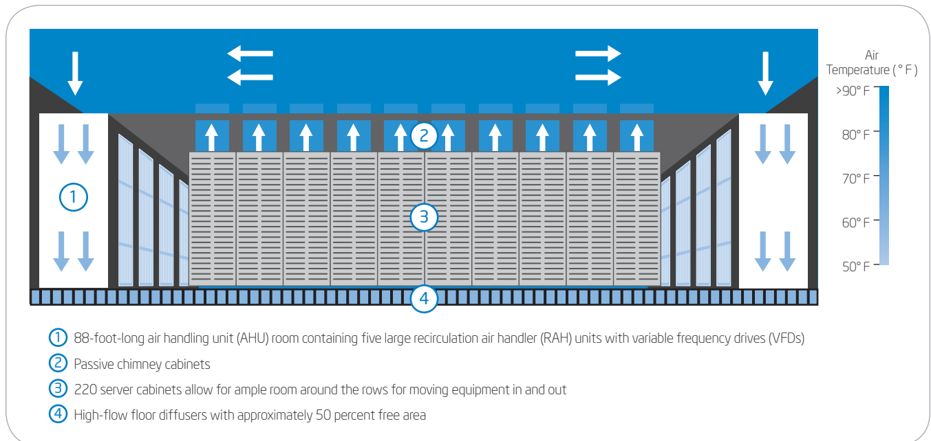
Figure 5. Model for a data center with 30 kilowatt cabinets.
