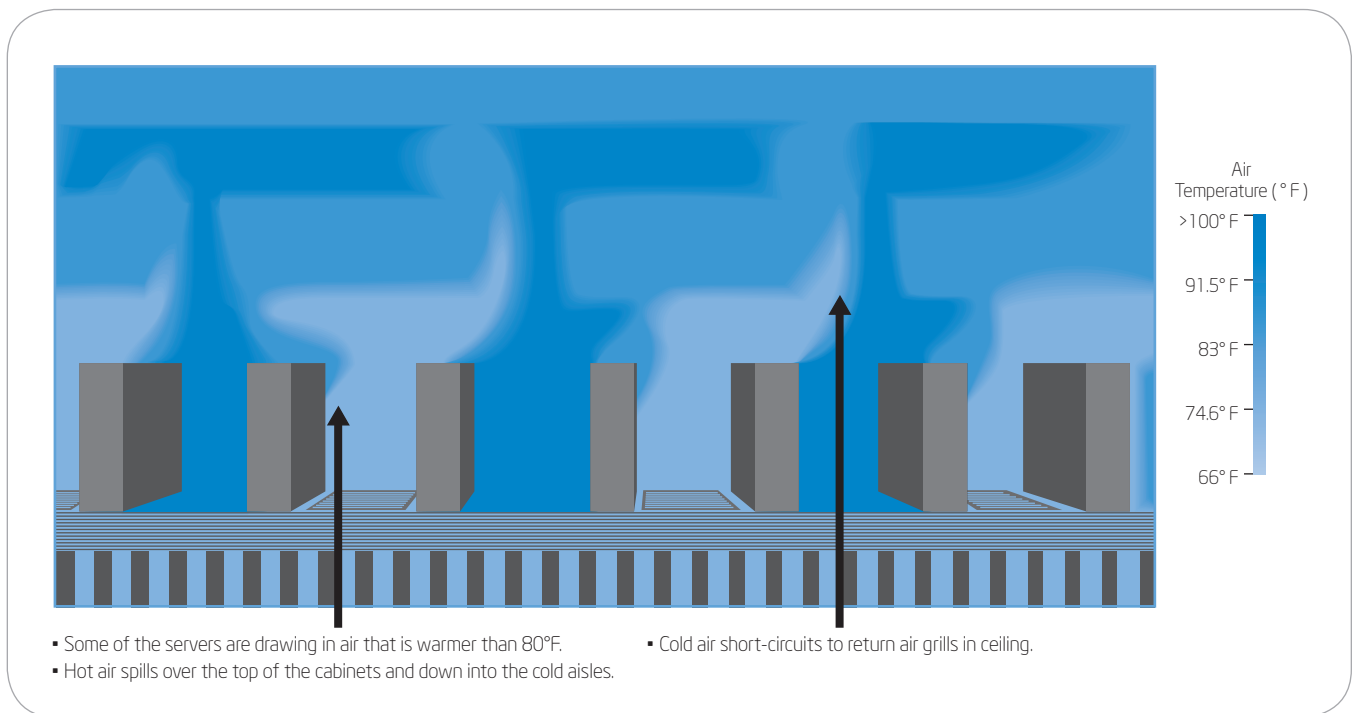
Figure 1. Hot air re-entrainment and cold air bypass in a data center without barriers between the aisles.
