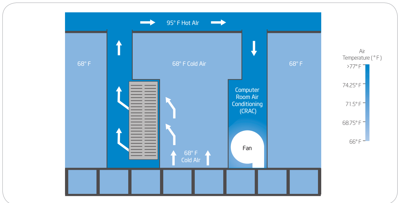
Figure 4. Passive chimney cabinets.
