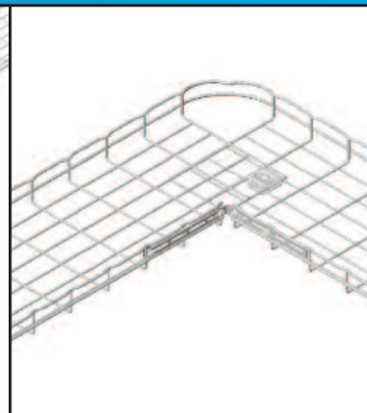
OnTrac® Splices, Turns & Supports
