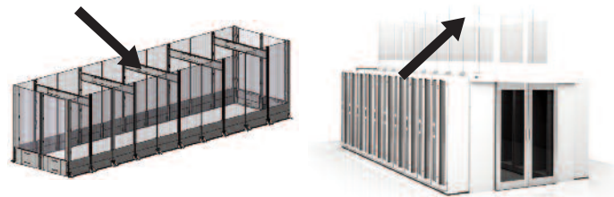
The images above show a completely assembled Cabinet Supported Exhaust Duct removed and installed on a row of cabinets. Cabinet Supported Exhaust Duct Horizontal Support Beams (five shown) connect the sides of the Cabinet Supported Exhaust Duct along the contained aisle. The Exhaust Duct also includes Exhaust Duct Panel Kits, End Panel Kits, H-Seal and Edge Seals.
