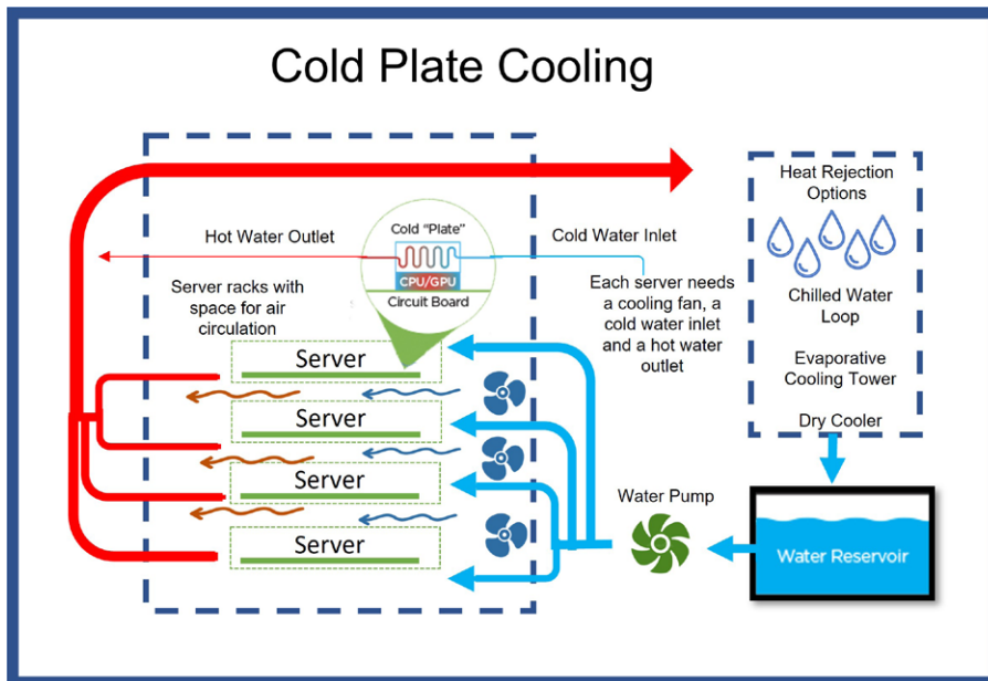
Figure 5: Direct to-chip, or cold plate, cooling solution
