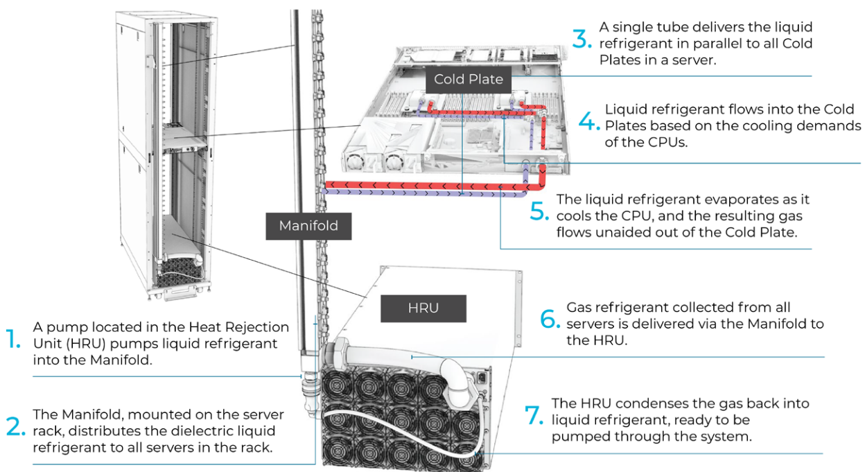
Figure 6: Two-phase direct to-chip, closed-loop dielectric liquid cooling solution with an air HRU
