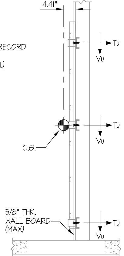
SIDE ELEVATION
